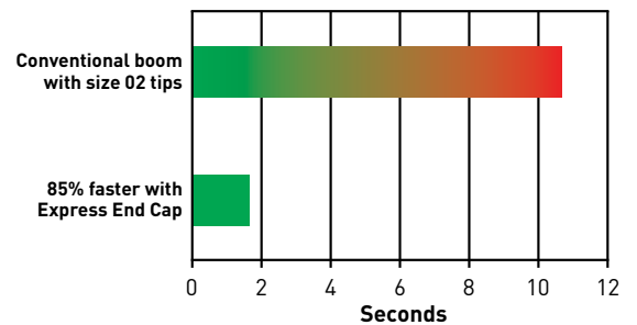
Reaction Time from "Close" Signal to Spray Stoppage
